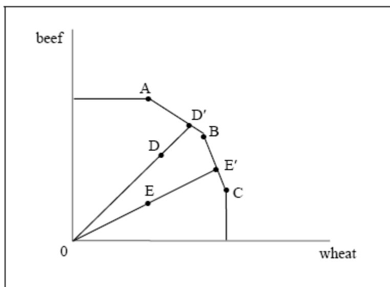
Figure 6 Output-Orientated DEA.
